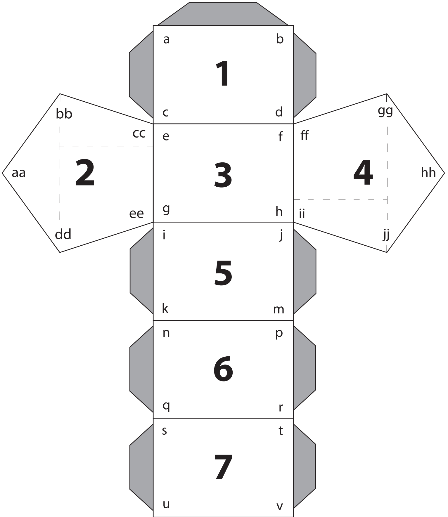
Pentagonal Prism
